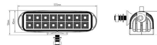
FARO A LED 12/24V 1732LM - 9W
