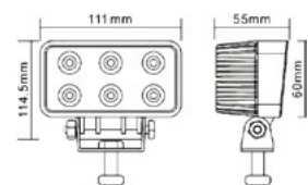
FARO A LED 12/24V 1100LM - 18W
