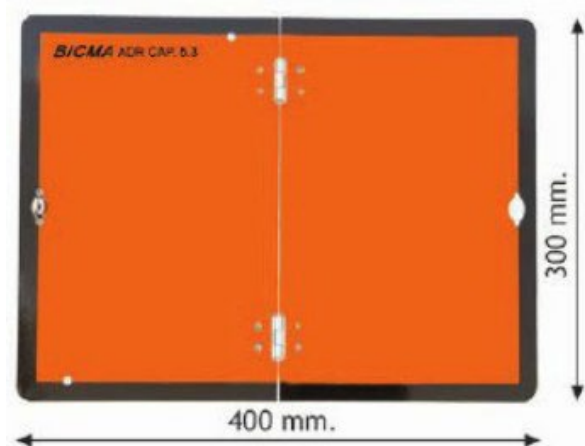
PANNELLO ADR Verticale
